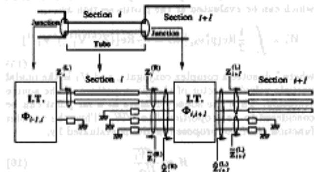
Figure 2. Equivalent electrical circuit.
