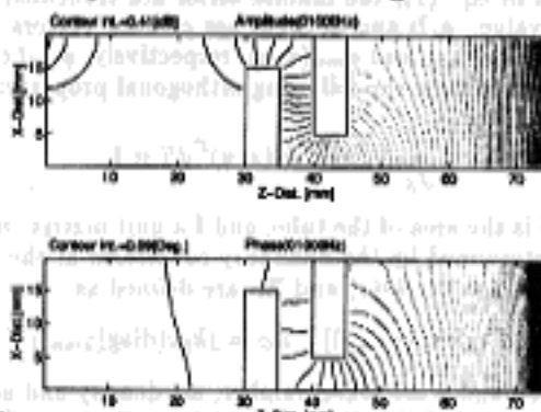
Figure 4. Sound-pressure distributions at 1kHz.
