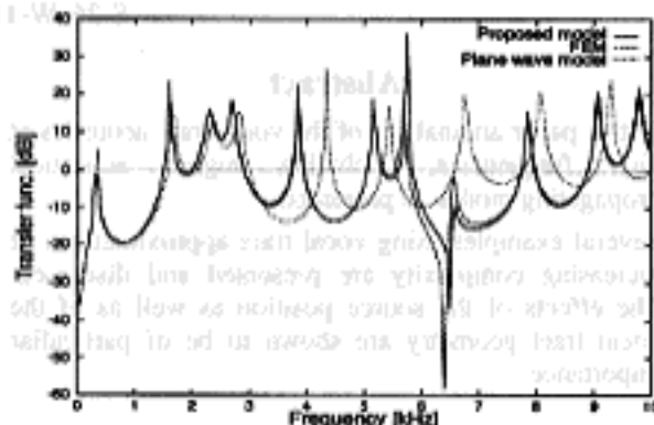
Figure 6. Transfer functions of 36-section configuration.
